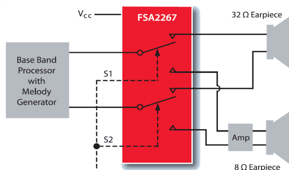
Figure 1. Application Diagram
