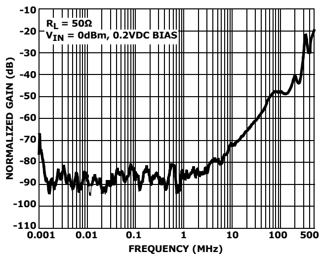
FIGURE 18. CROSSTALK
