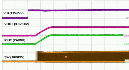
Startup Through V IN 2A Load
