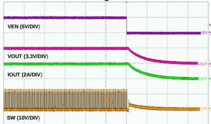
Shutdown Through V EN 2A Load
