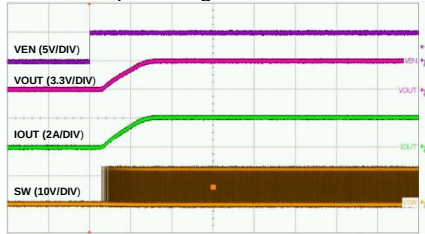
Startup Through V EN 2A Load
