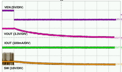
Shutdown Through V EN 0A Load
