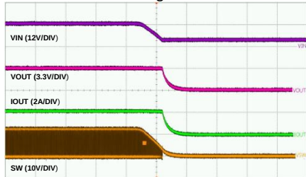
Shutdown Through V IN 2A Load
