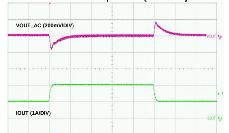
Transient Response (1 to 2A)
