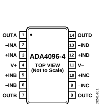
Figure 6. 14-Lead TSSOP (RU-14), ADA4096-4
