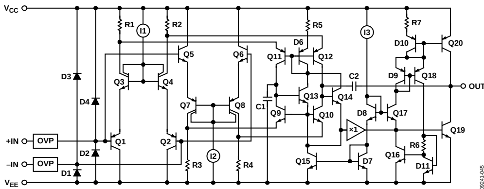
Figure 53. Simplified Schematic, ADA4096-2
