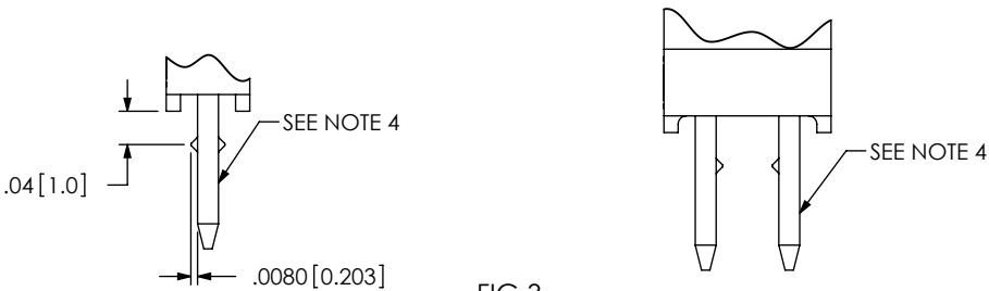
FIG 3 LOCKING LEAD OPTION (DIMS APPLY TO BOTH -S AND -D)
