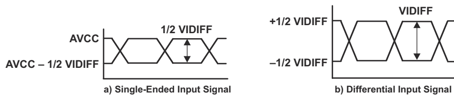
Figure 9-2. TMDs Inputs
