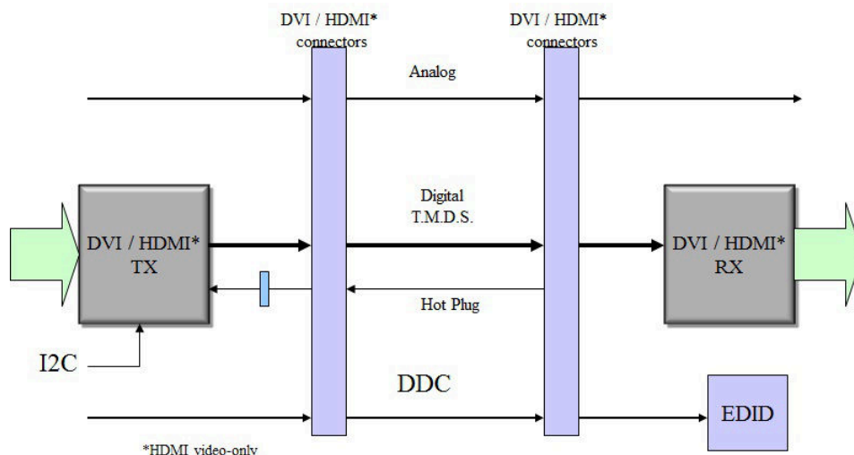
TFP401 Diagram
