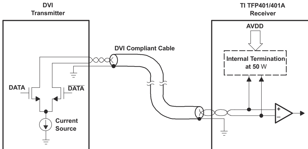
Figure 9-1. TMDs Differential Input and Transmitter Connection
