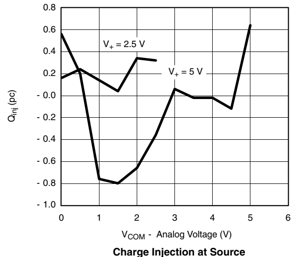
Charge Injection at Source
