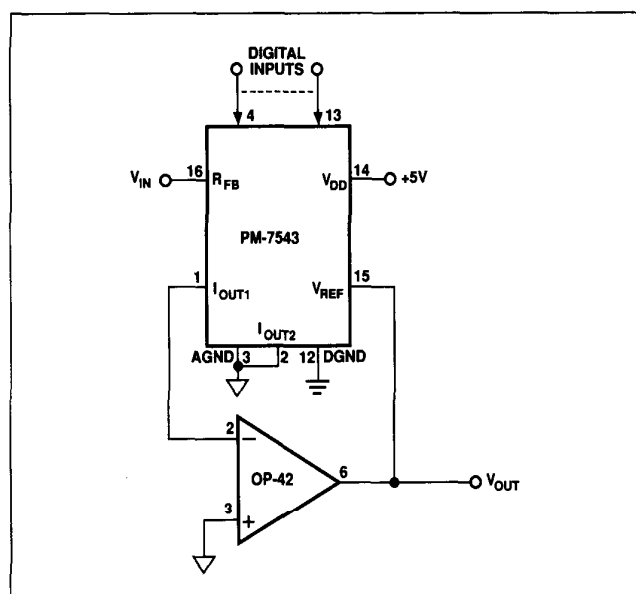
FIGURE 10: Analog/Digital Divider
