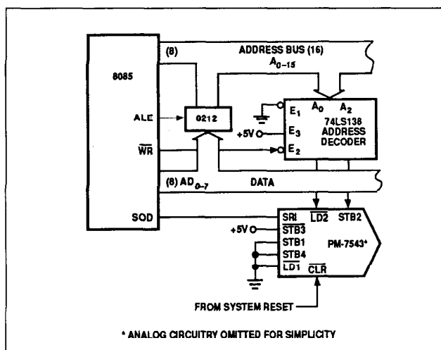
FIGURE 12: PM-7543 - 8085 Interface
