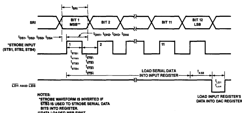
FIGURE 6: Timing Diagram
