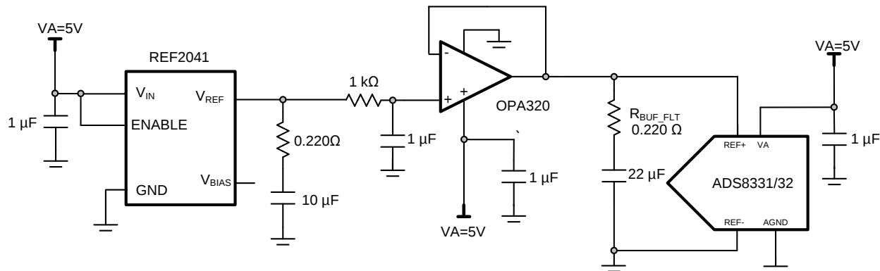
Figure 50. Reference Driver Schematic for V_A = 5 \text{ V} , V_{\text{REF}} = 4.096 \text{ V}
