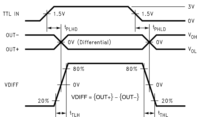
Figure 7-4. Differential Driver Propagation Delay and Transition Time Waveforms
