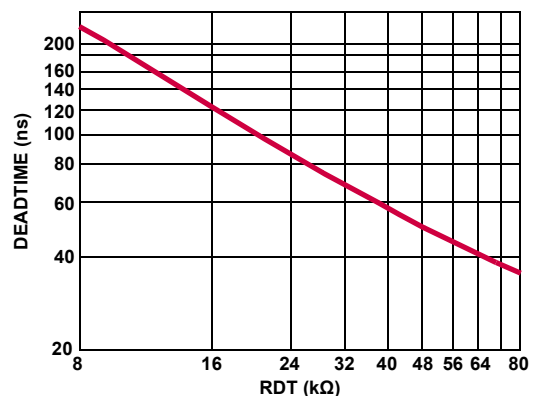
FIGURE 2. DEAD-TIME vs TIMING RESISTOR
