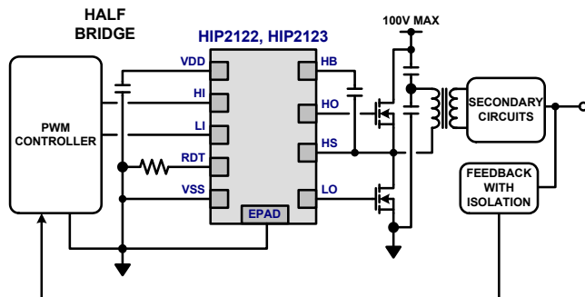
FIGURE 1. TYPICAL APPLICATION
