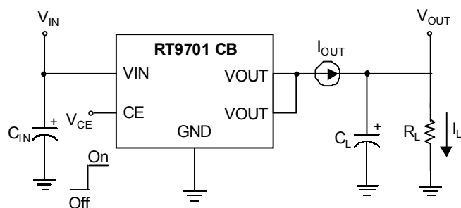
Test Circuit 3
