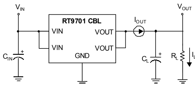
Test Circuit 1
