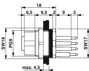
M12 flush-type socket, contact length: 12 mm
