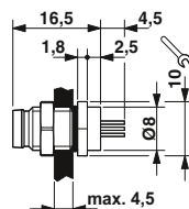
M8 flush-type plug
