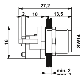
M12 flush-type plug, straight,
