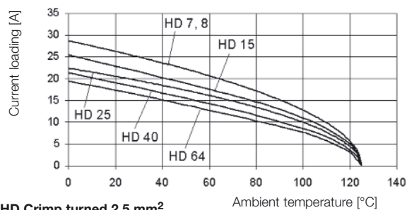
HD Crimp turned 2.5 mm 2
