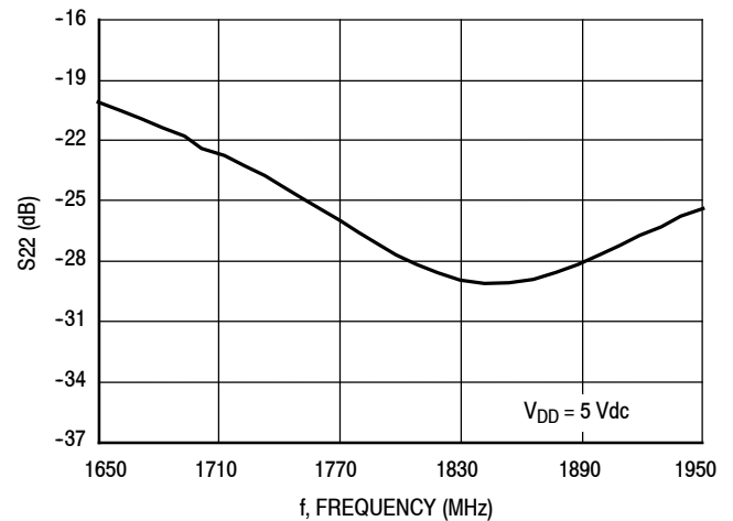
Figure 18. S22 versus Frequency
