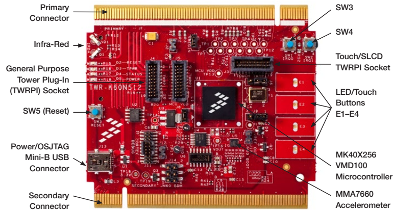
Figure 1: Front Side of TWR-K40X256 Board Not Including TWRPI
