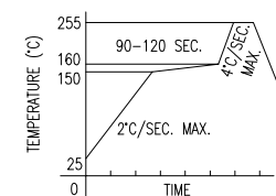
C LEAD FREE REFLOW PROFILE 10 SEC. MAX.
