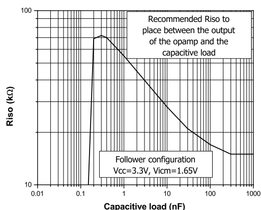
Figure 30. In-series resistor ( R_{iso} ) vs. capacitive load
