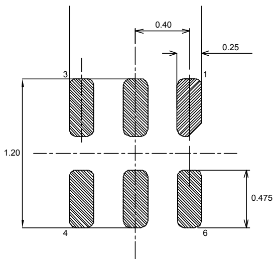
Figure 41. DFN6 1.2x1.3 recommended footprint
