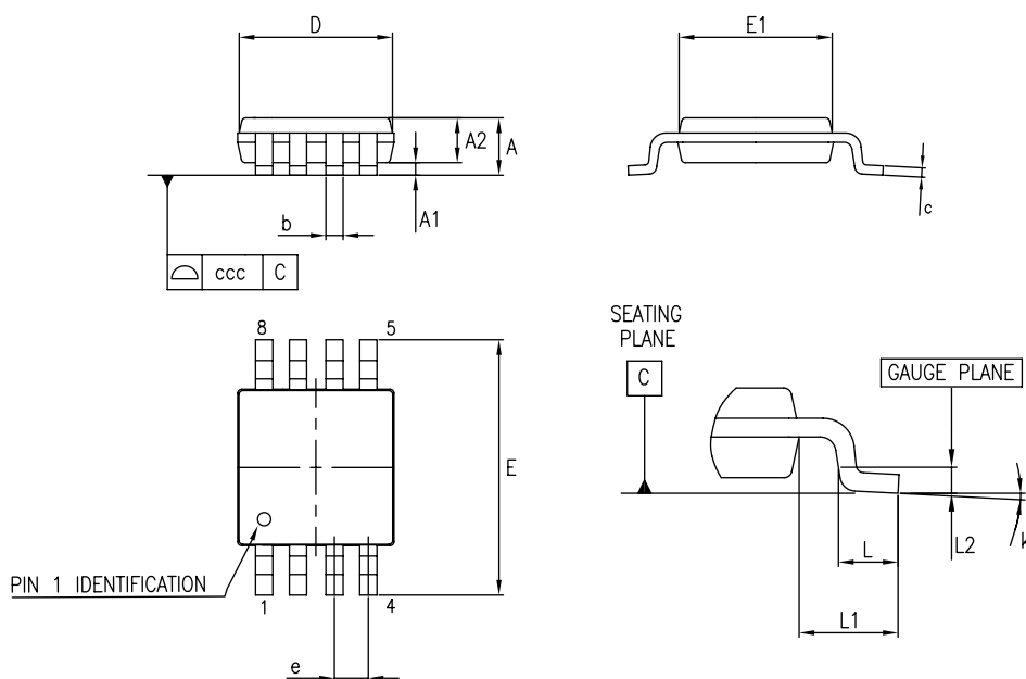
Figure 42. MiniSO8 package outline
