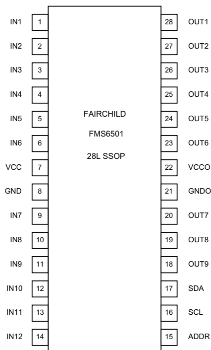
Figure 2. Pin Configuration
