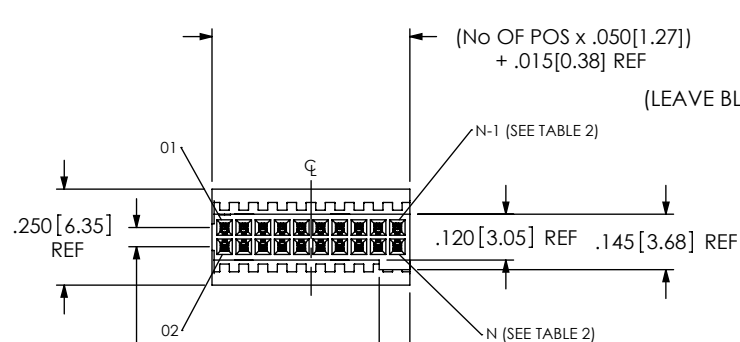
FIG. 1 -S: SINGLE END (SFSD-10-28-XX-XX.XX-S SHOWN)
