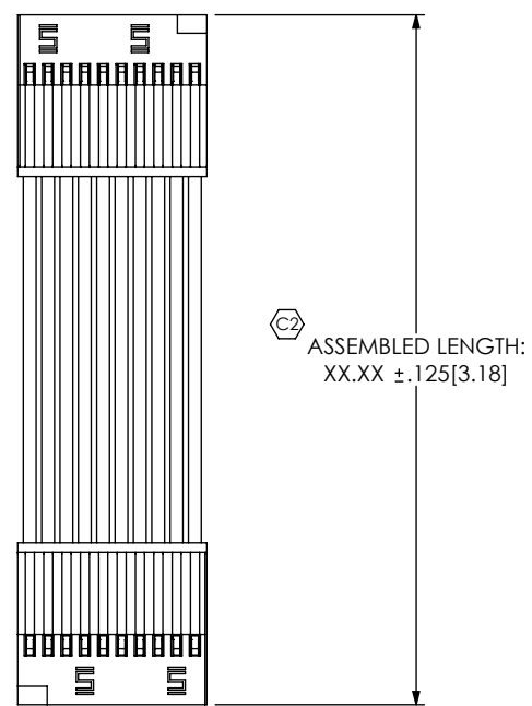
FIG. 2 -D: DOUBLE END (SFSD-10-28-XX-XX.XX-D-NUS SHOWN) (SAME AS FIG. 1, UNLESS OTHERWISE STATED)
