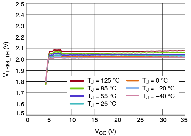
Figure 26. Trigger Threshold
