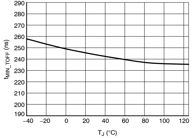
Figure 34. Minimum Off-time R_{MIN\_TOFF} = 0\ \Omega
