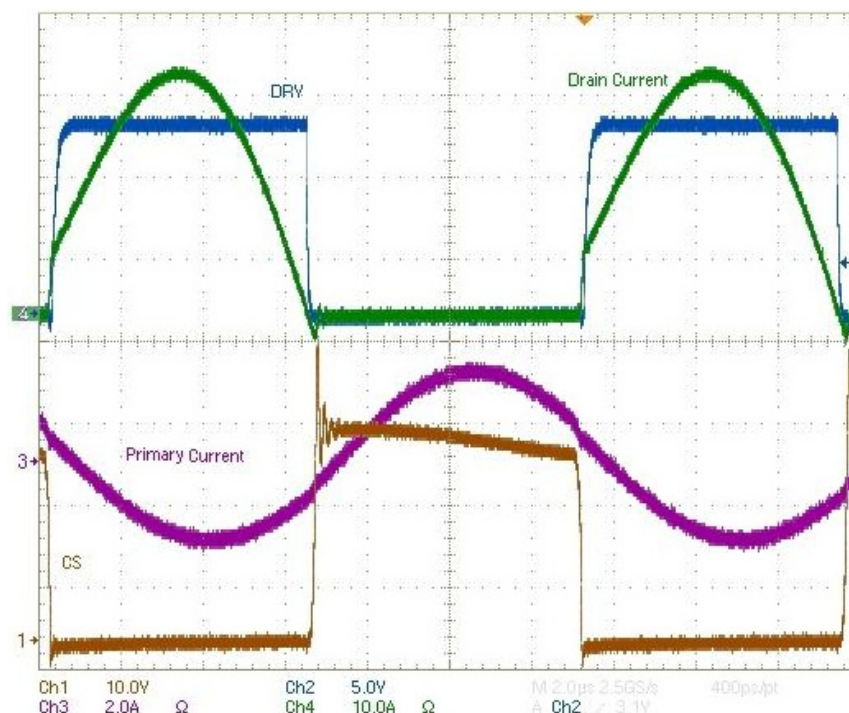
Figure 49. Waveforms from SR System Implemented in LLC Application and Using MOSFET in SMT Package with Minimized Parasitic Inductance – SR MOSFET Channel Conduction Time is Optimized
