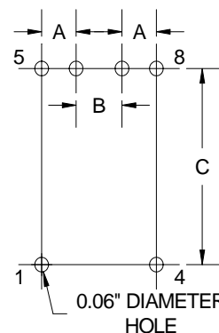
Board Layout
