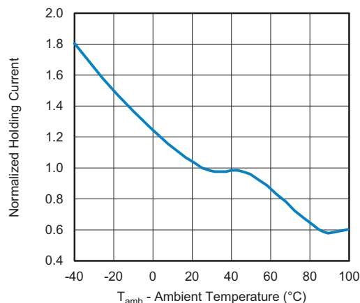
Fig. 6 - Normalized Holding Current vs. Ambient Temperature
