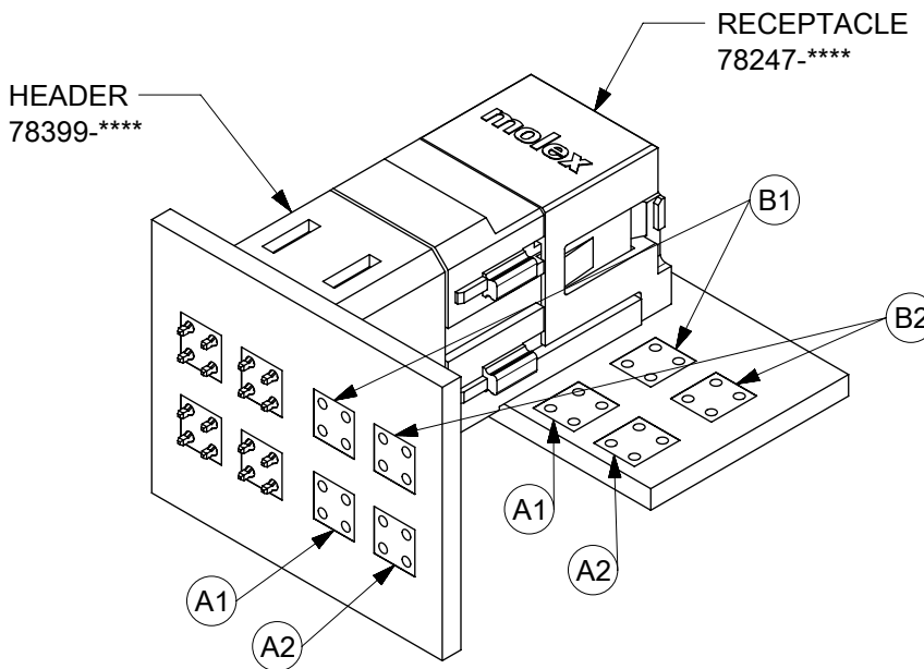
VERTICAL HEADER (78399) & RIGHT-ANGLE RECEPTACLE (78247)
