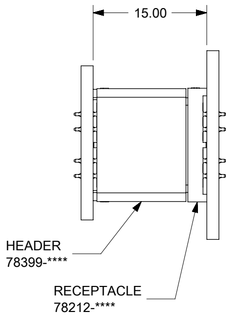
VERTICAL HEADER (78399) & VERTICAL RECEPTACLE (78212)
