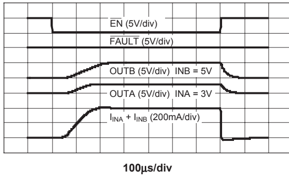
Turn-ON/OFF Response with 20\Omega 1\mu\text{F} loads
