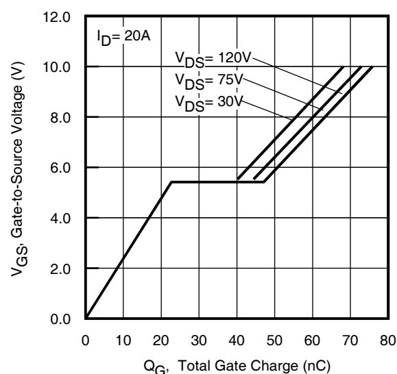
Fig 10. Typical Gate Charge vs. Gate-to-Source Voltage
