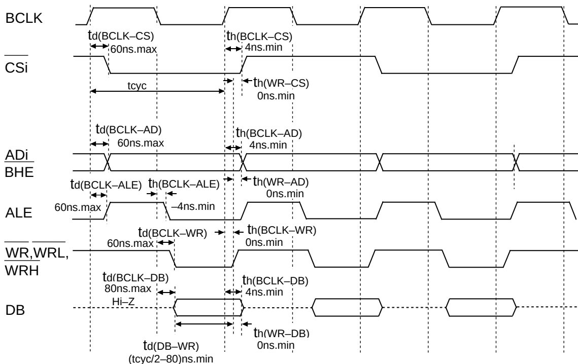
Figure 1.26.4. Timing diagram (3)
