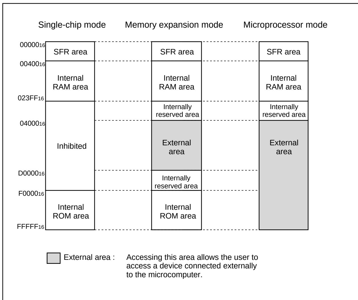
Figure 1.7.2. Memory maps in each processor mode
