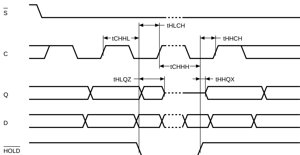
Figure 18. Hold Timing
