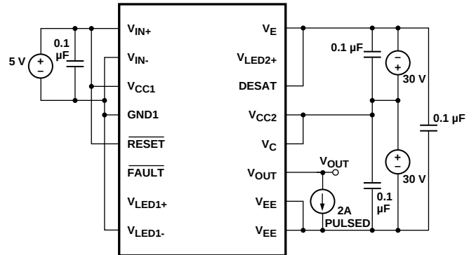
Figure 35. V_{\text{OH}} Pulsed Test Circuit.
