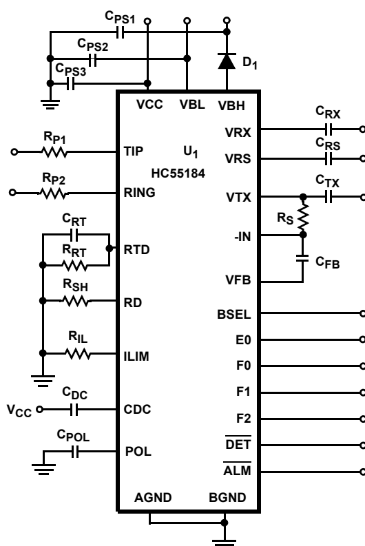
FIGURE 15. HC55184 BASIC APPLICATION CIRCUIT
