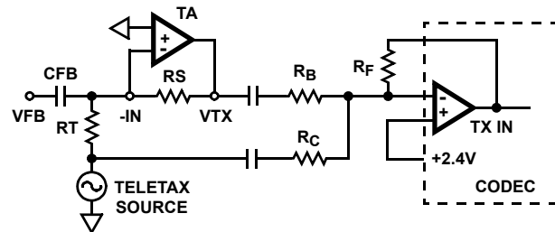
FIGURE 18. TELETAX SIGNALLING
