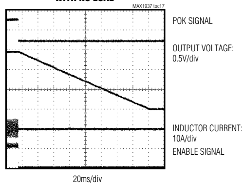
SHUTDOWN WAVEFORM WITH NO LOAD
