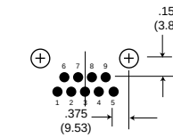
9 Contacts
