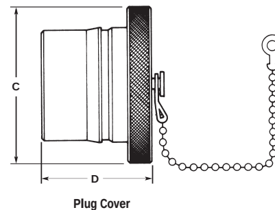
Plug Cover
