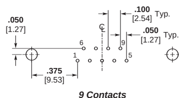
9 Contacts
