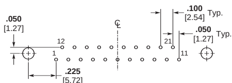
21 Contacts
