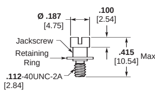
Part Number 6-1532137-2 Jackscrew Assembly Low Profile (J) 096-0002-0062 M83513/5-15 (JM) S96-0002-0089
