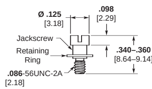
Part Number 5-1532137-7 Jackscrew Assembly Low Profile (L) 096-0002-0011 M83513/5-05 (LM) S96-0002-0085
