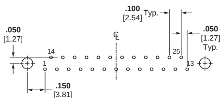
25 Contacts
