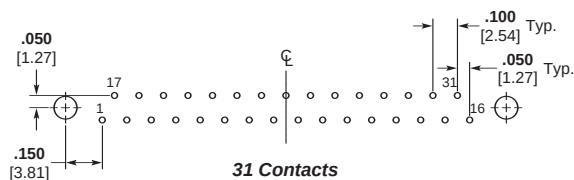
31 Contacts
