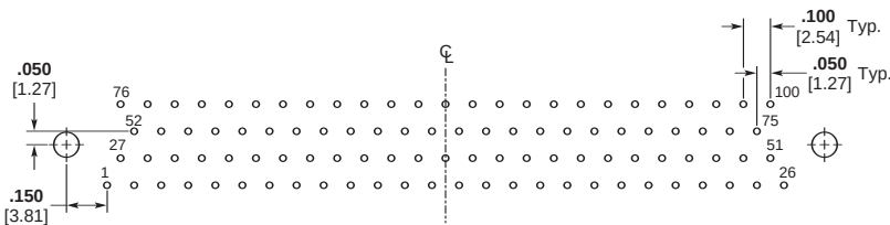
100 Contacts
