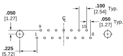
15 Contacts
