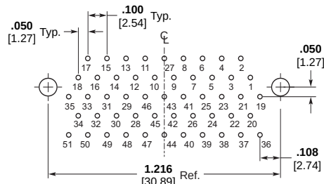
51 Contacts
