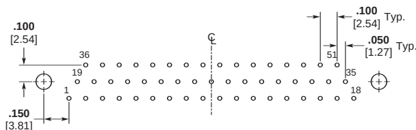
51 Contacts
