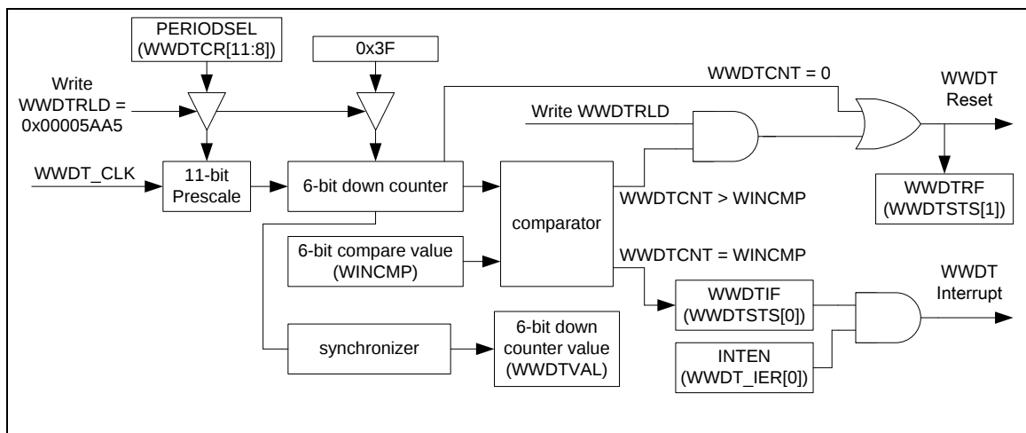
Figure 5-131 Watchdog Controller Block Diagram
