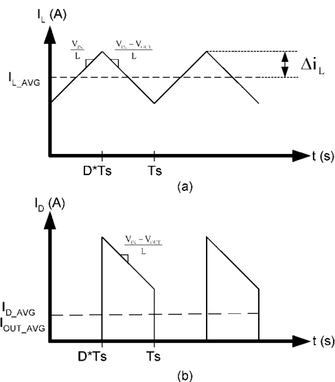
FIGURE 5. (a) Inductor current. (b) Diode current.
