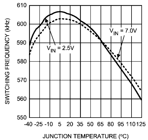
660kHz Switching Frequency vs. Temperature
