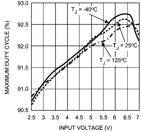
660kHz Max. Duty Cycle vs. Input Voltage
