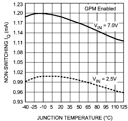
Non-Switching Quiescent Current vs. Temperature GPM Enabled
