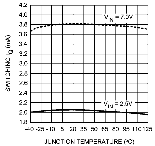
660kHz Switching Quiescent Current vs. Temperature
