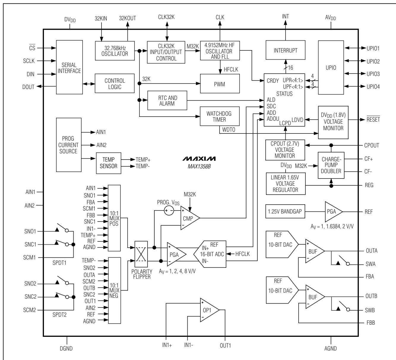
Figure 3. Functional Diagram
