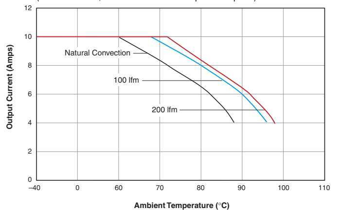
LSN-1.8/10-D12 Output Current vs. Ambient Temperature (Vertical mount, air flow direction from pin 11 to pin 1)
