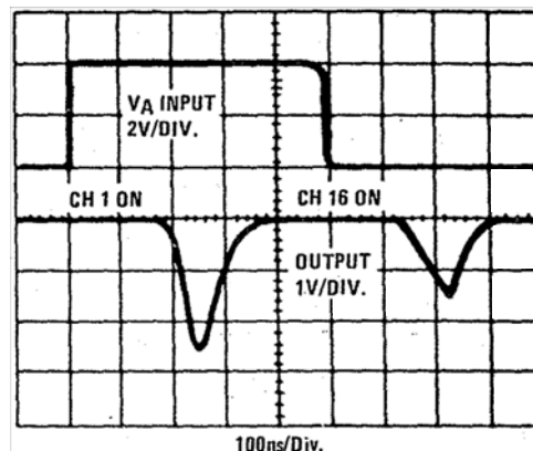
BREAK-BEFORE-MAKE DELAY ( t_{\text{OPEN}} )
