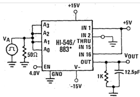
BREAK-BEFORE-MAKE DELAY ( t_{\text{OPEN}} )
