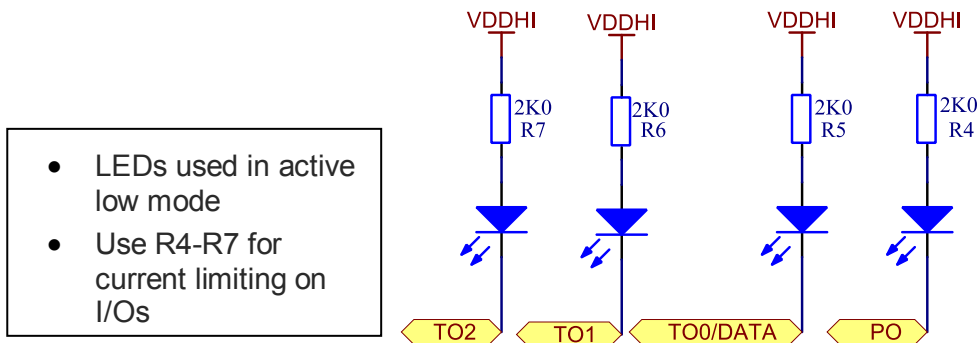
Figure 4.1 Reference Design for IQS133. Output in active Low.
