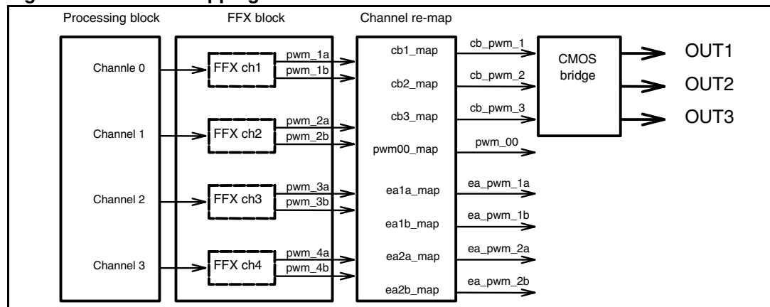
Figure 25. FFX re-mapping
