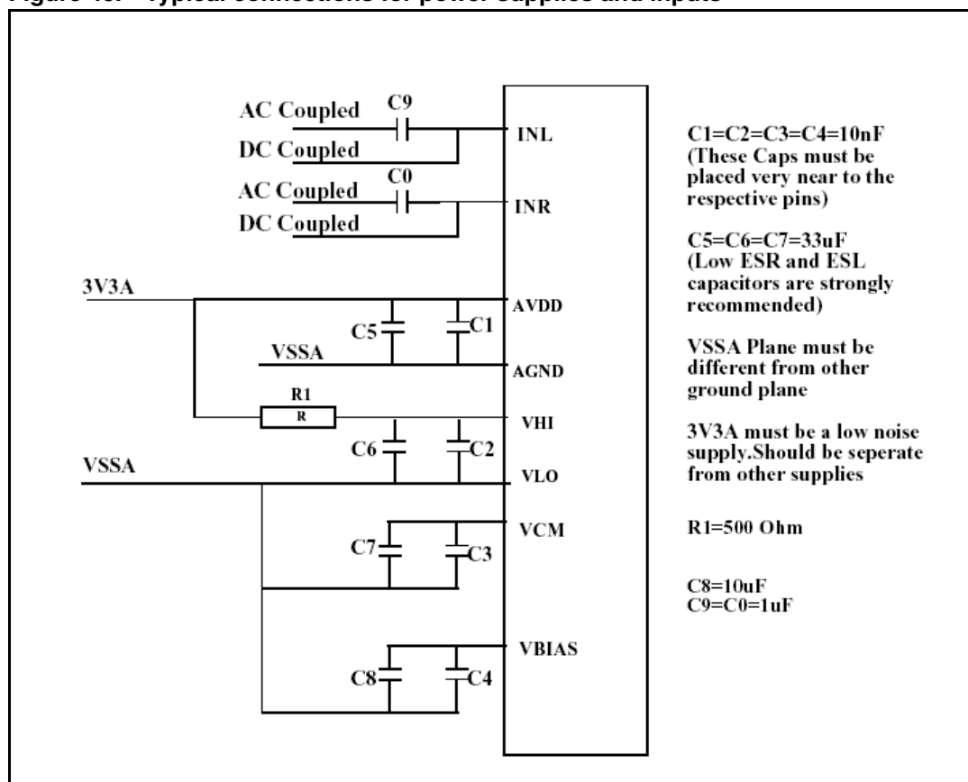
Figure 40. Typical connections for power supplies and inputs
