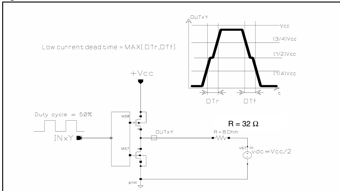
Figure 3. Test circuit
