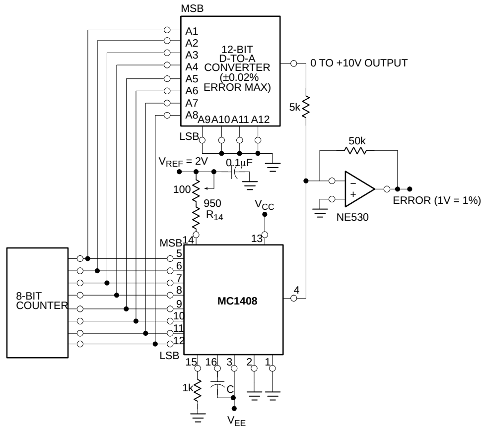
Figure 5. Relative Accuracy
