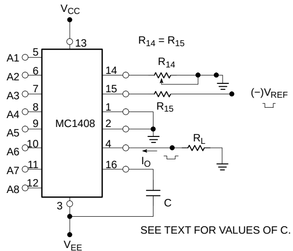
Figure 4. Negative V_{REF}
