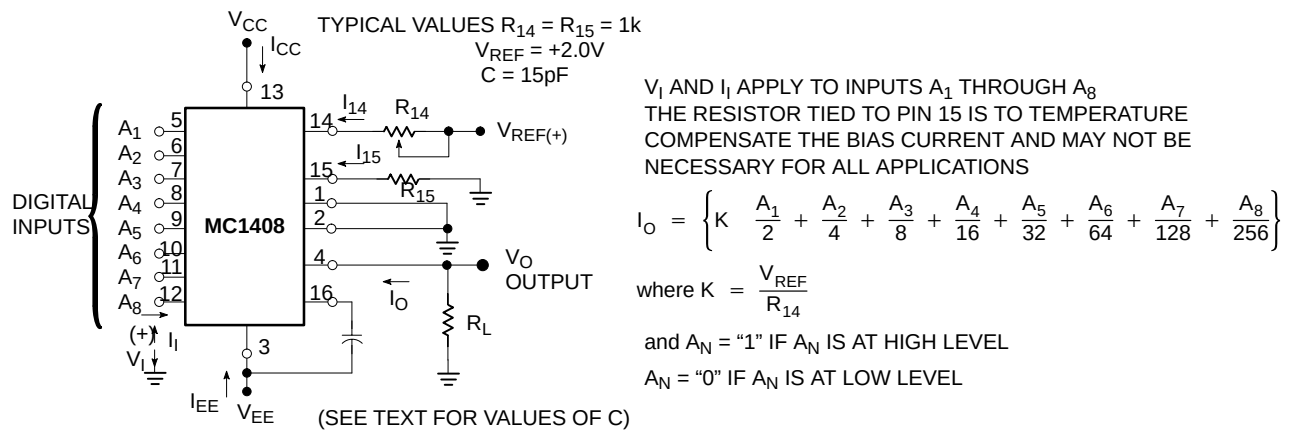
Figure 7. Notation Definitions
