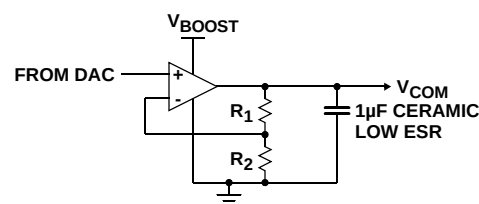
FIGURE 24. V COM USED AS A BUFFER WITH GAIN
