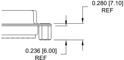
02 ..... 0.236" BOARD SIDE
