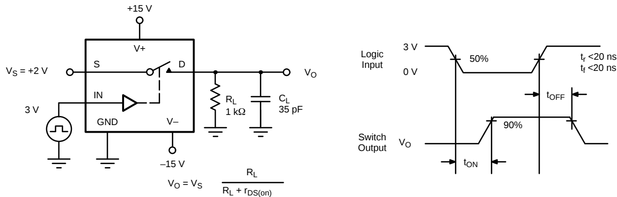
FIGURE 2. Switching Time
