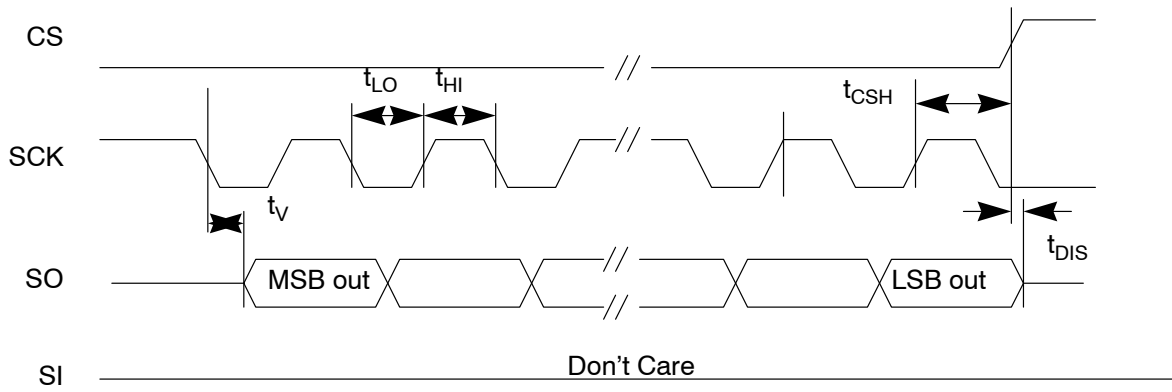
Figure 16. SPI Output Timing
