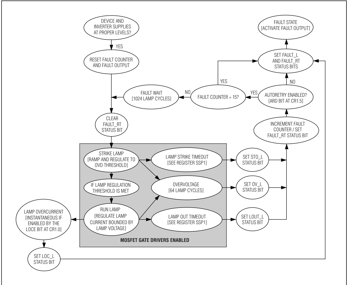
Figure 8. Fault-Handling Flowchart
