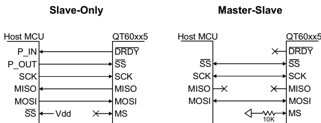
Figure 4-1 SPI Connections
