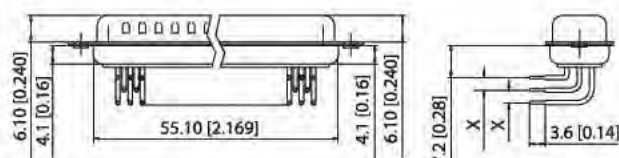
50 Positions Machined Pin (W/O Rear Cover)
