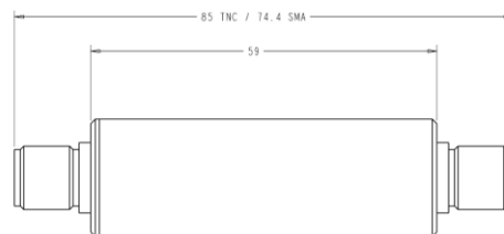
TW126 Dimensions (mm)
