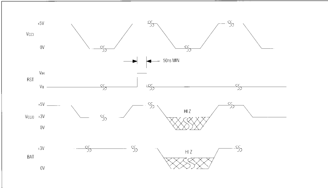
Figure 4. Reset Timing
